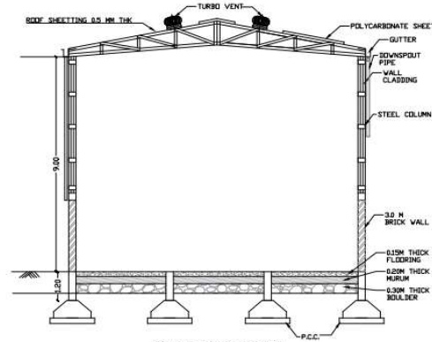
SECTION X-X' SCALE 1:100
