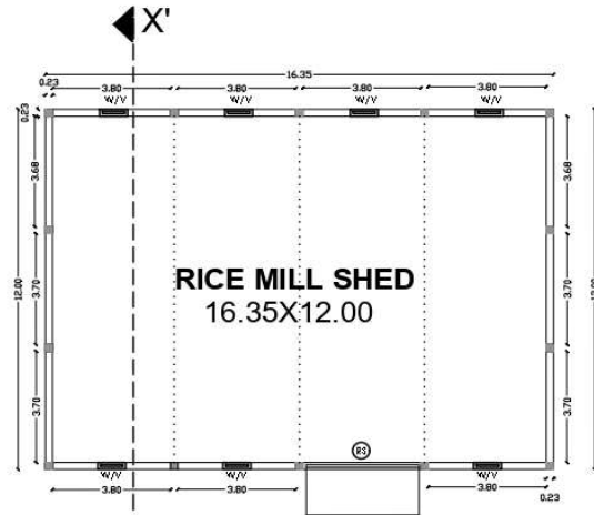
PROPOSED RICE MILL SHED PLAN SCALE 1:100
