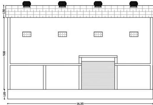
PROPOSED ELEVATION SCALE 1:100
