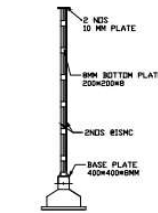
ISMC COLUMN
